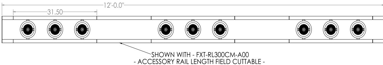
ASSEMBLY WITH THREE 393 FIXTURES AND ACCESSORY RAIL KIT
