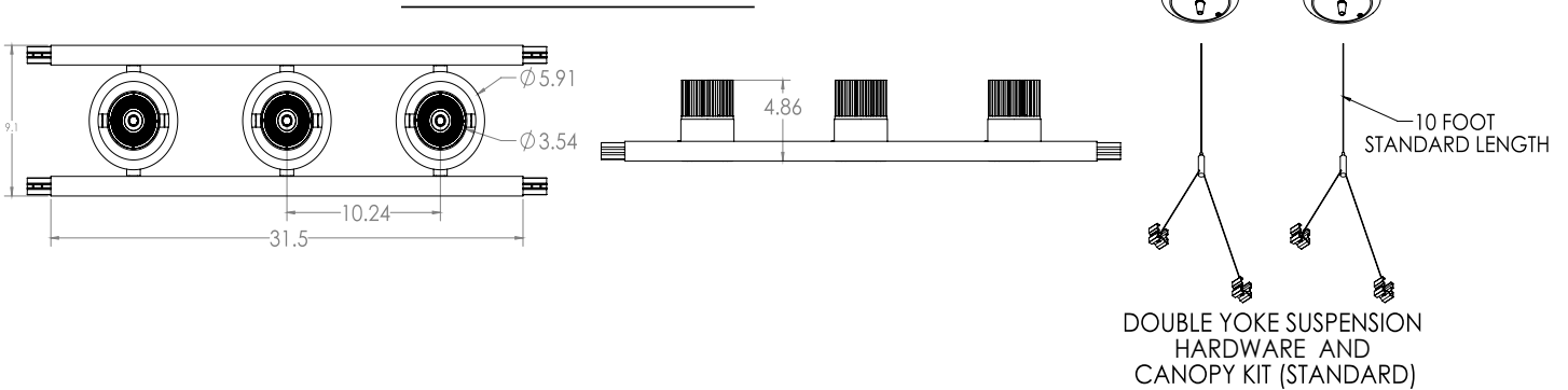
Example: 393 Fixture Dimensions
