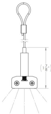
Hanging Mount (HM)
