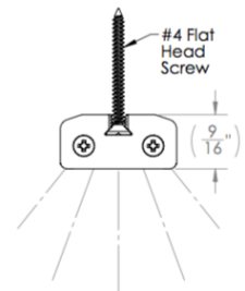
Surface Mount (SM)
